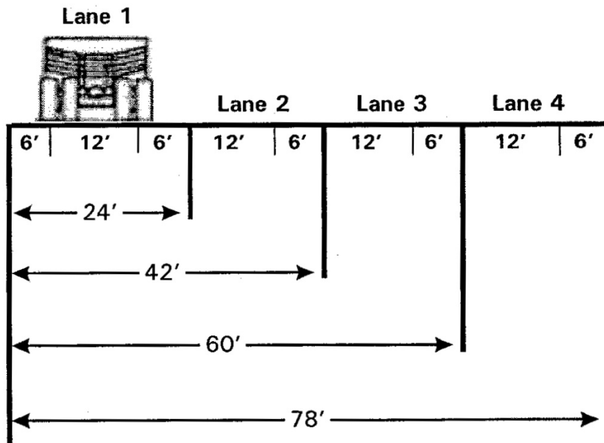
Typical haulageway sections for 12-foot-wide vehicle
